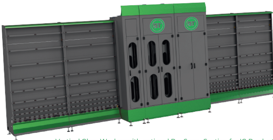
Vertical Glass Washer with optional Pre Spray Section for IG Production
